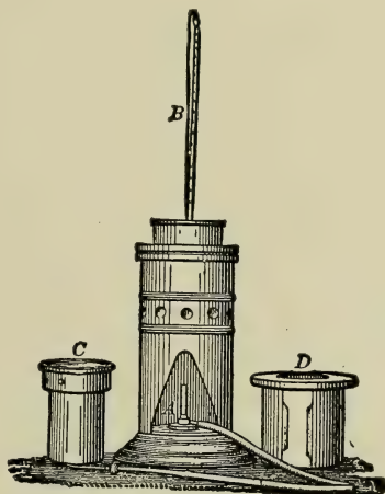
FIG. 184.—New York State Closed Flash-point Tester.
